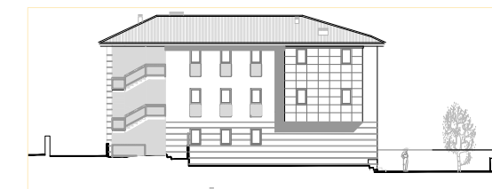
ALZADO PRINCIPAL
